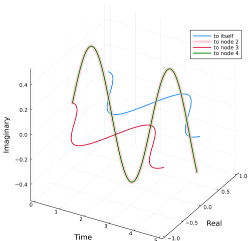
Figure 6: Probability amplitudes of node 1's wave function are complex...
